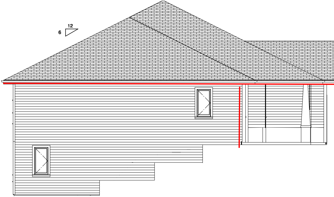
LEFT ELEVATION
