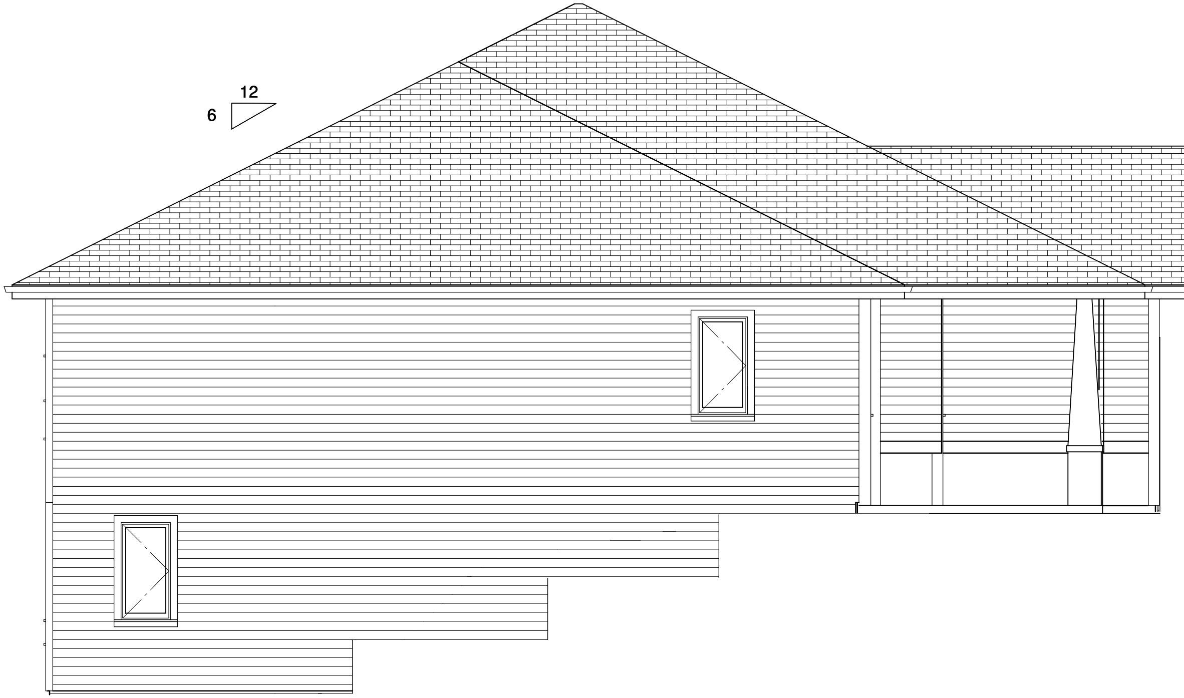
LEFT ELEVATION
